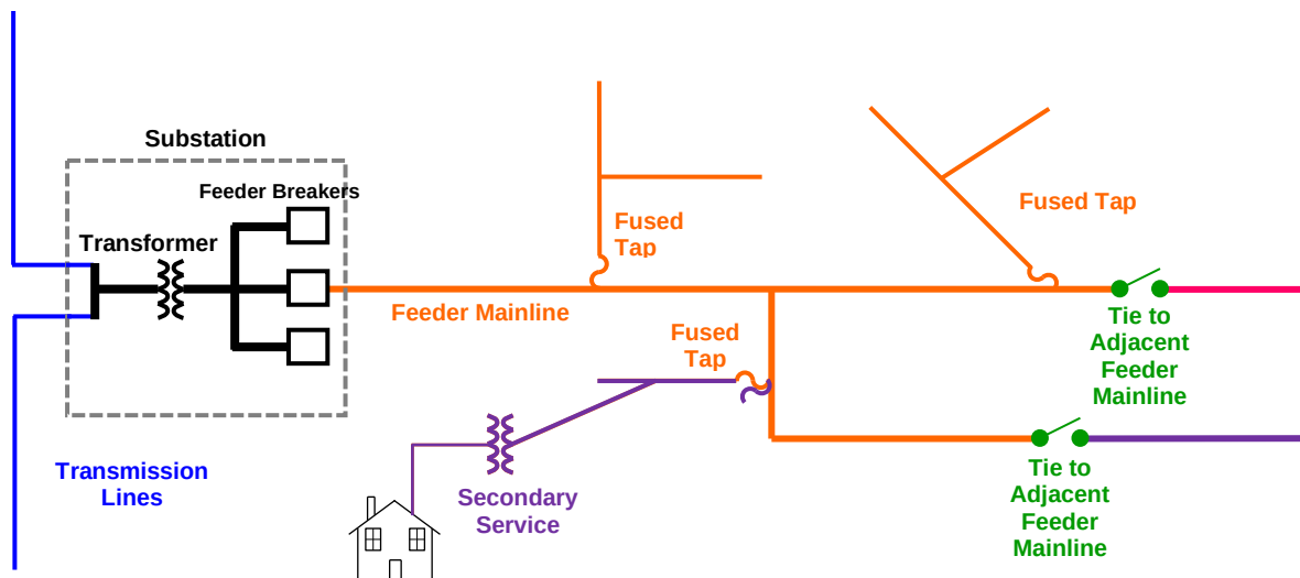
Figure 2: Distribution System: Basic Design Schematic of Typical Radial Circuit Design
