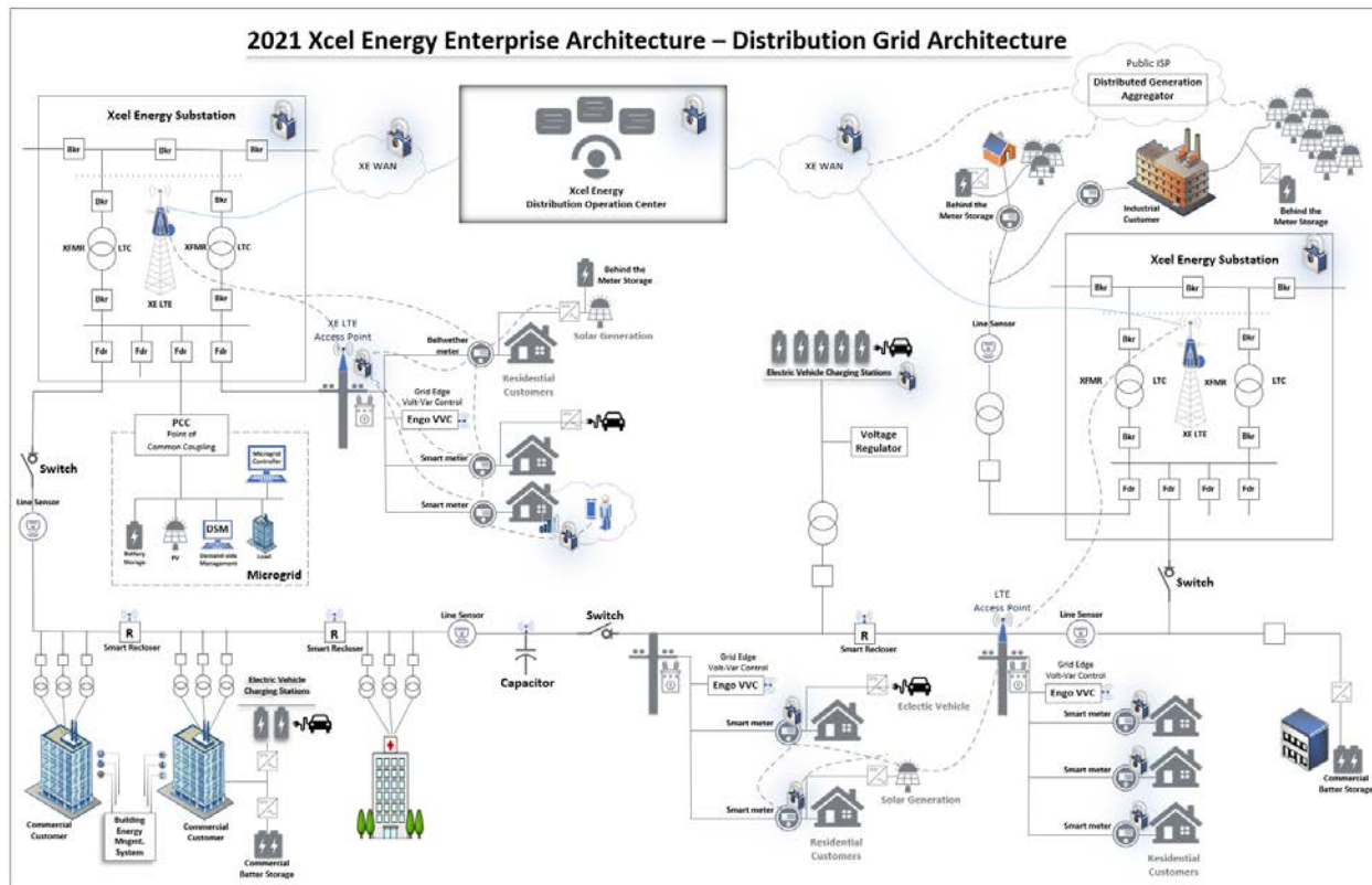
Figure 4: Xcel Energy Enterprise Architecture – Distribution Grid Architecture
