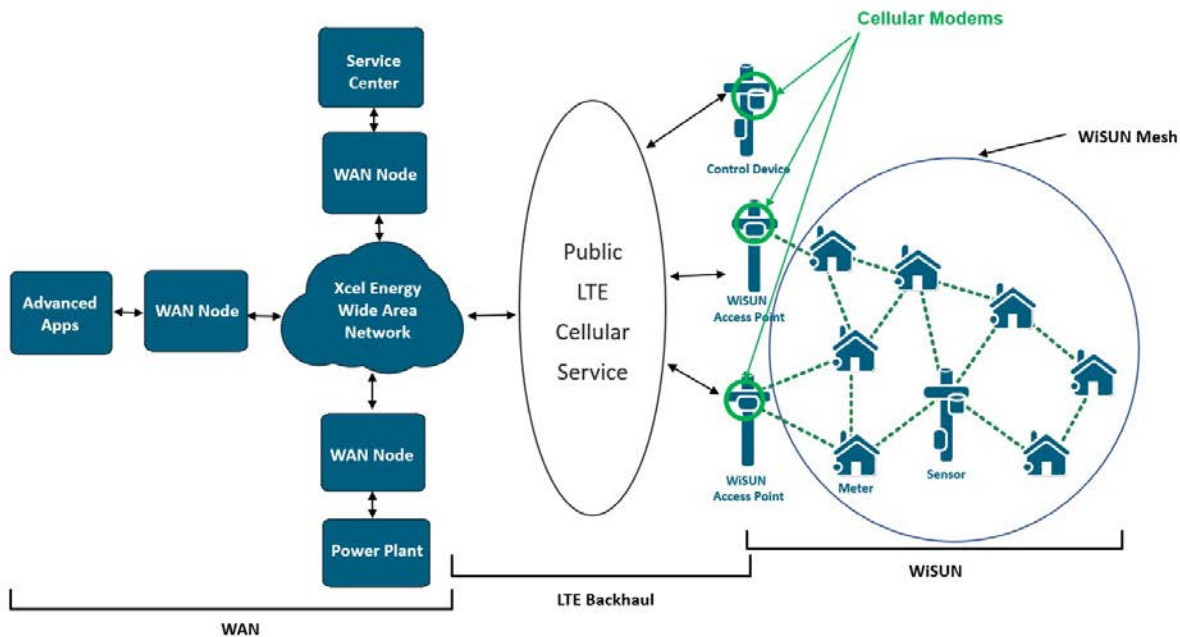
Figure 5: Field Area Network Illustration
