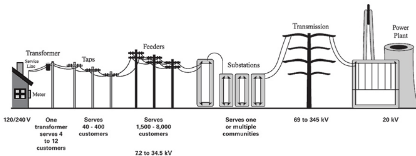
Figure 1: Major Grid Components
