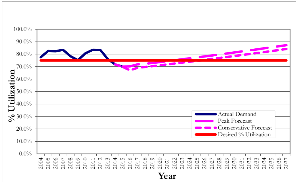
Figure 6: Illustrative Total Feeder Circuit Utilization in Study Area – Historical Peak Demand and Peak Demand Forecast
