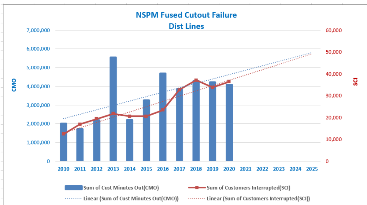
Figure 3: NSPM Fused Cutout Failures 2010-2020
