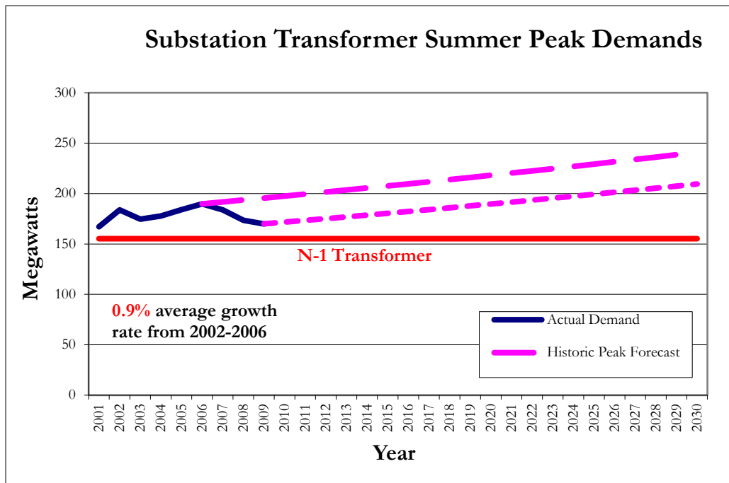
Figure 8: Illustrative Greater Study Area – Historical and Forecasted Loads
