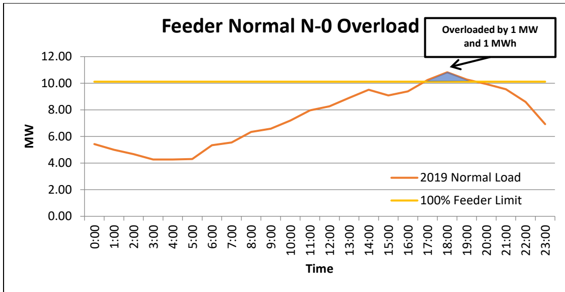
Figure 1: Illustrative N-0 Overload
