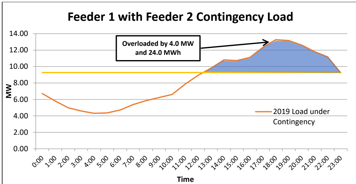
Figure 2: Peak Day Load Curve for Feeder 1 after Feeder 2 Second Section Load has been Transferred
