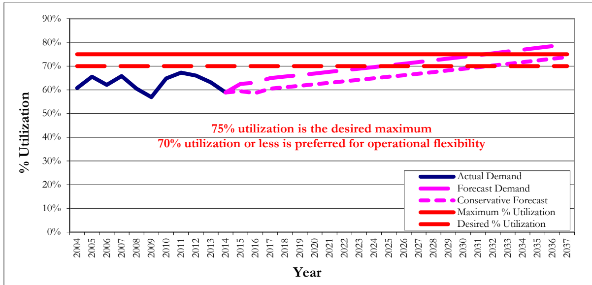
Figure 9: Illustrative Total Transformer Utilization Percentage for Transformers – Focused Study Area
