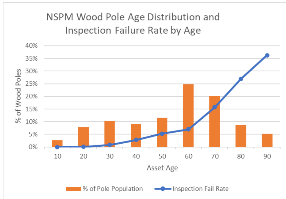
Figure 1: NSPM Wood Pole Inspection Failures by Age
