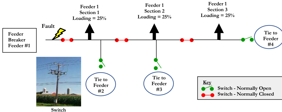
Figure 4: Typical Mainline Distribution Feeder with Three Sections Capable of System Intact N-0 and First Contingency N-1 Operations Mainline Feeder No. 1
